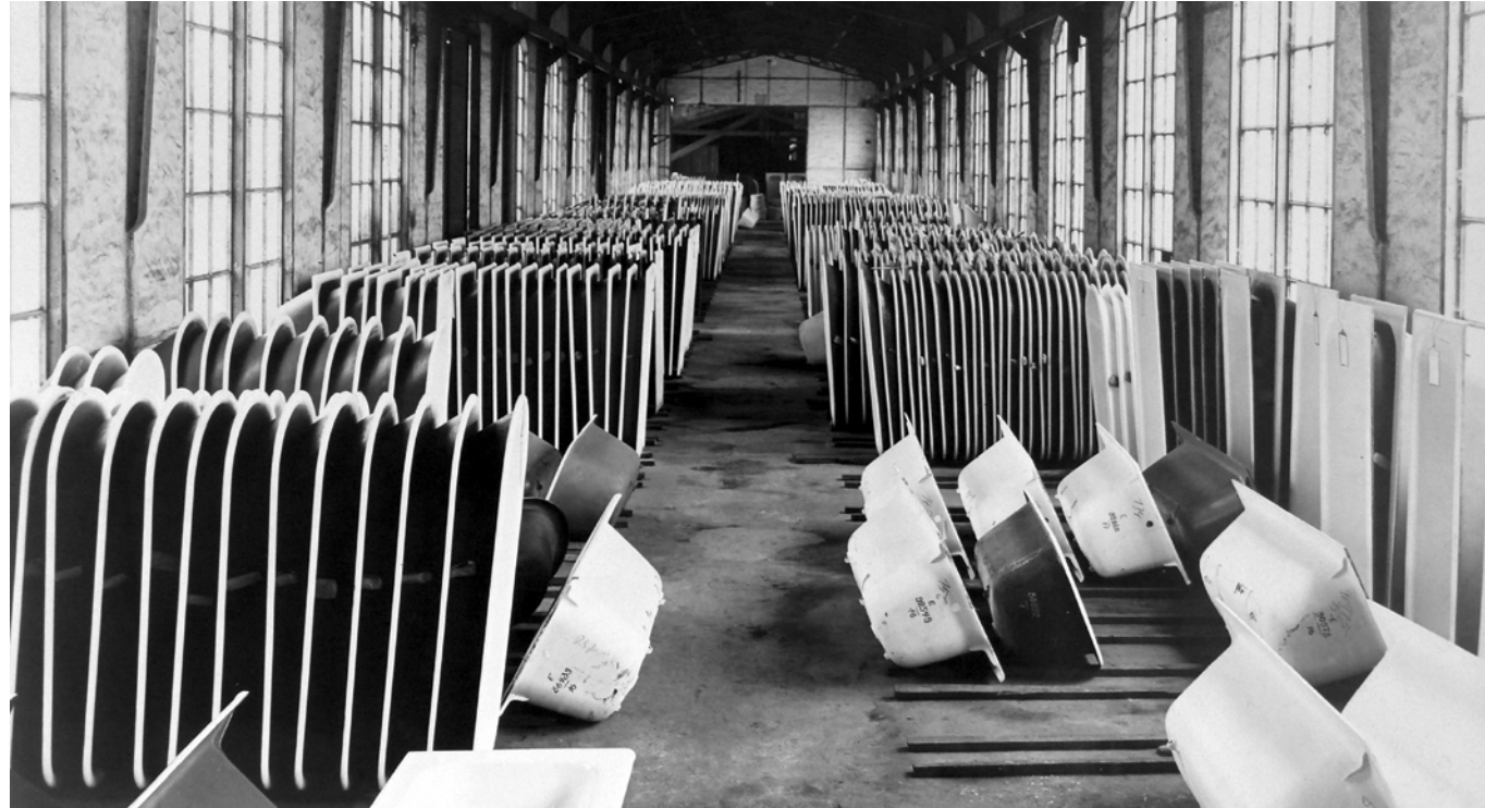
Produktionshalle der Guss-Badewannen um 1927 Production hall for cast iron bathtubs about 1927
